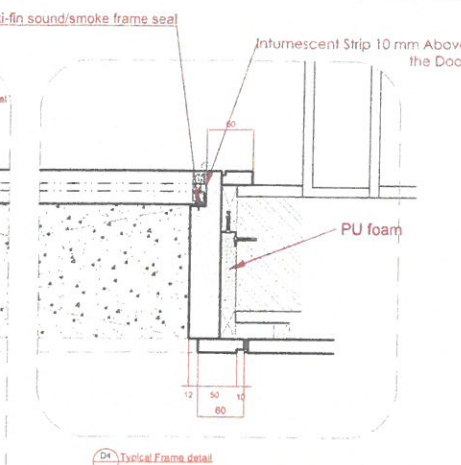
D4 Typical Frame detail
